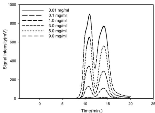
Fig. 5. Chromatograms of loxoprofen racemate at different sample concentrations from SMB columns packed with CHI-II CSP, (sample loading amount=100 \mu l, mobile phase flow rate=3.0 ml/min, mobile phase=n-hexane/Et-OH/acetic acid=99/1/0.1).
